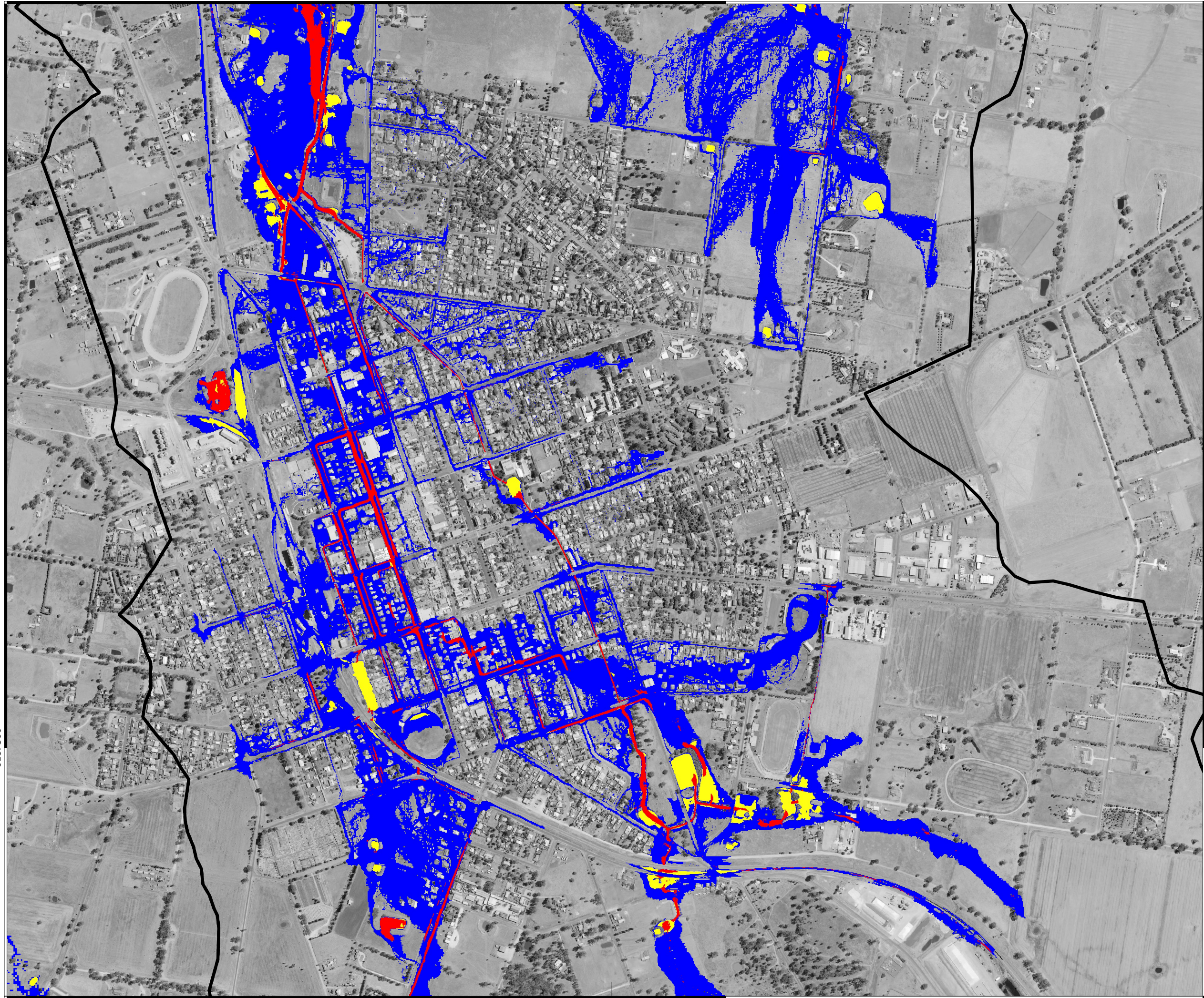
Figure 24B: Design Results - Hydraulic Categories - 1% AEP Event
